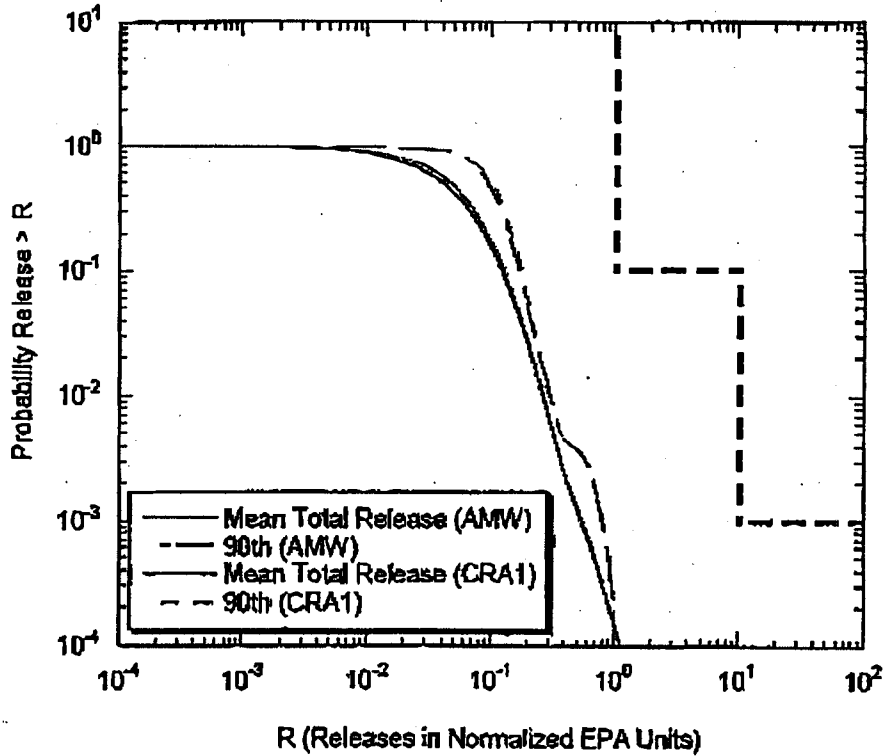
Figure 2. Comparison of AMW PA total releases with releases from the modified Compliance Recertification Application (CRA1). The CRA1 uses the PAVT spillings modeling instead of the spillings model used in the forthcoming (~March 26, 2004) CRA. (Source: Hansen et al. 2004, Docket A-98-49, Item II-B2-30)
